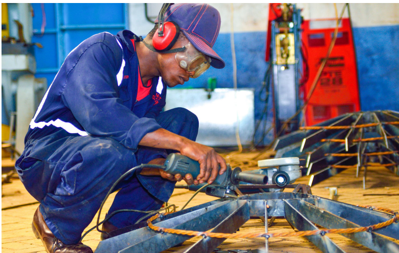
Street lighting pole fabrication
